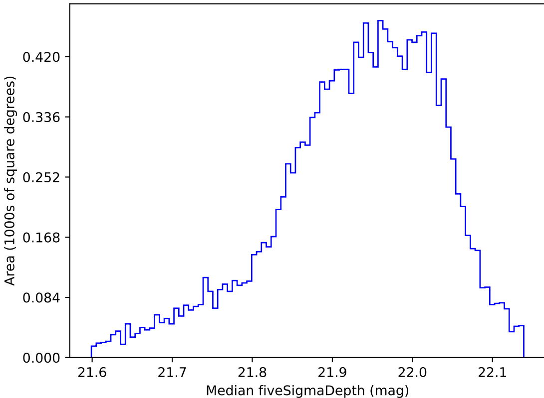
baseline_v2.1_10yrs WFD y band: Median fiveSigmaDepth
