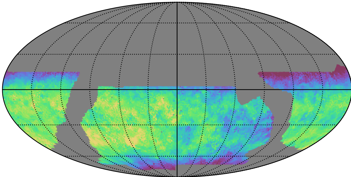
baseline_v2.1_10yrs WFD u band: Median fiveSigmaDepth
