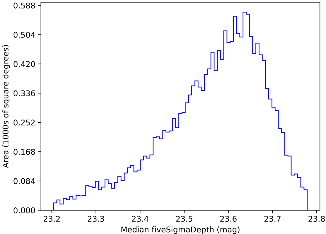
baseline_v2.1_10yrs WFD u band: Median fiveSigmaDepth
