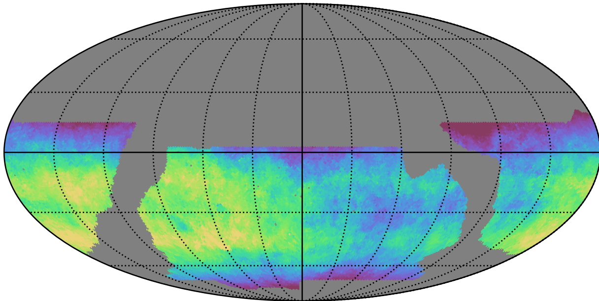
baseline_v2.1_10yrs WFD r band: Median fiveSigmaDepth
