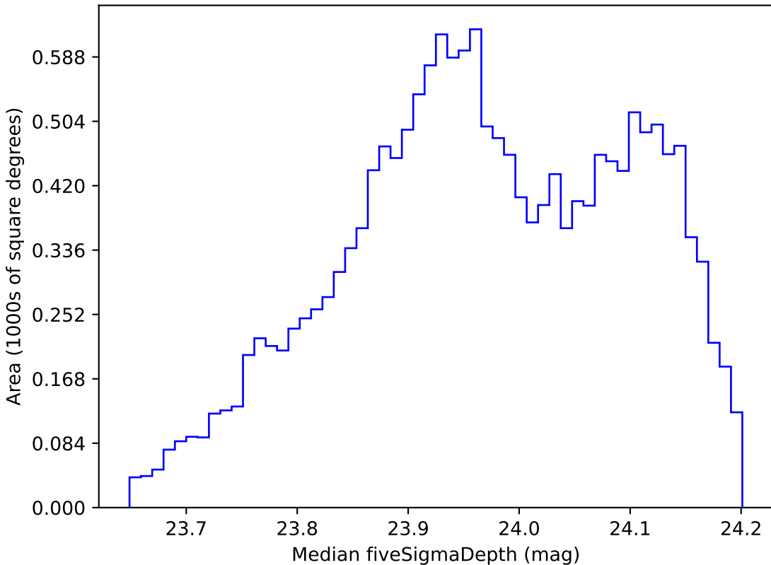
baseline_v2.1_10yrs WFD r band: Median fiveSigmaDepth
