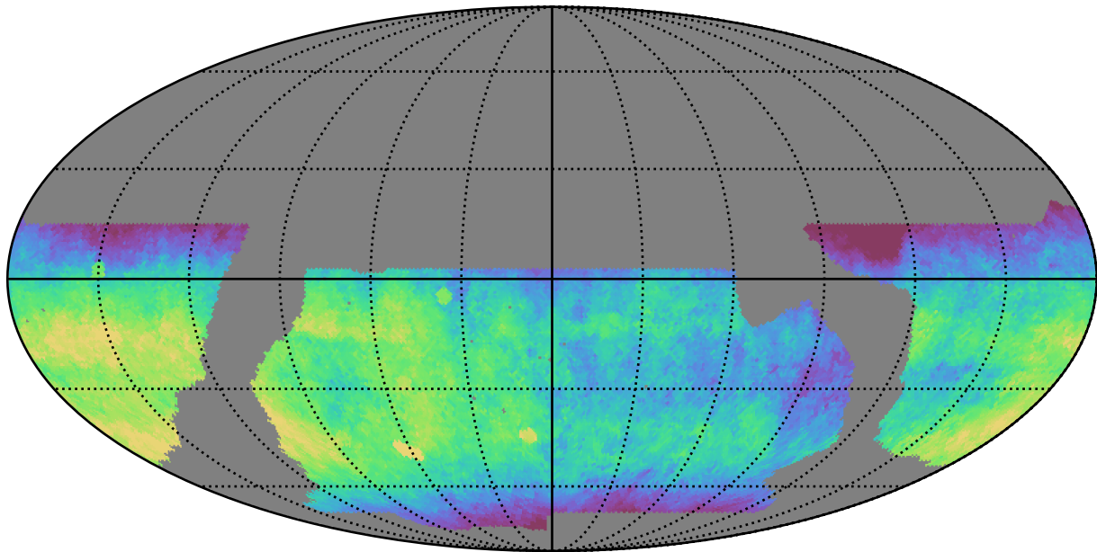
baseline_v2.1_10yrs WFD i band: Median fiveSigmaDepth
