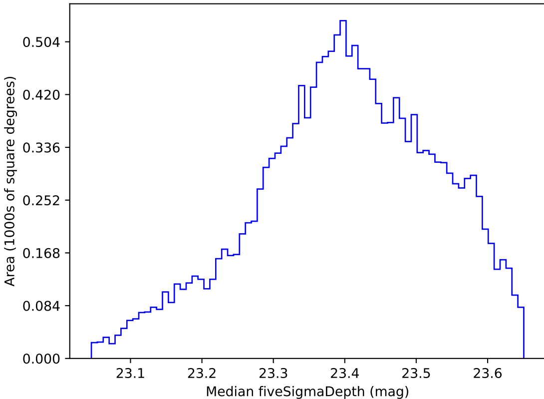
baseline_v2.1_10yrs WFD i band: Median fiveSigmaDepth
