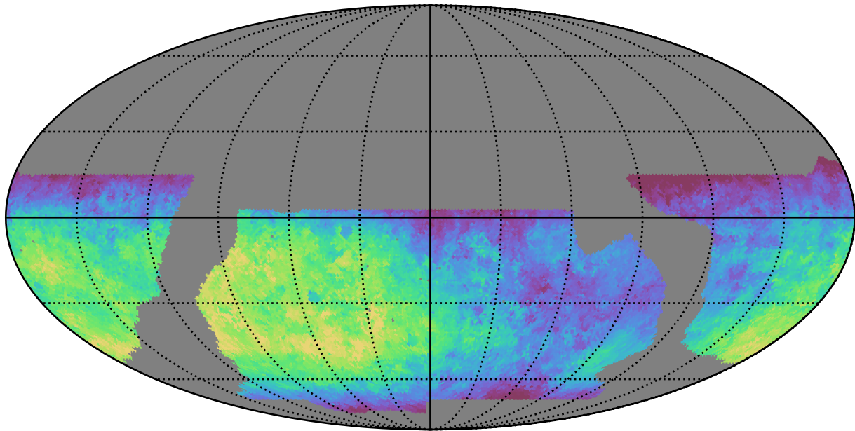
baseline_v2.1_10yrs WFD g band: Median fiveSigmaDepth
