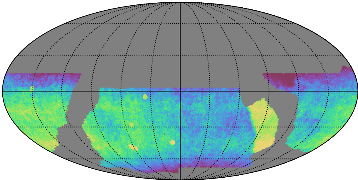
baseline_v2.1_10yrs WFD all bands: Median fiveSigmaDepth
