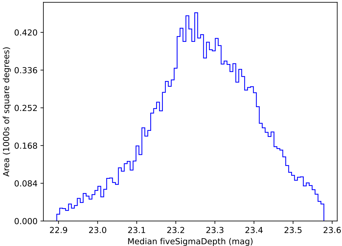
baseline_v2.1_10yrs WFD all bands: Median fiveSigmaDepth
