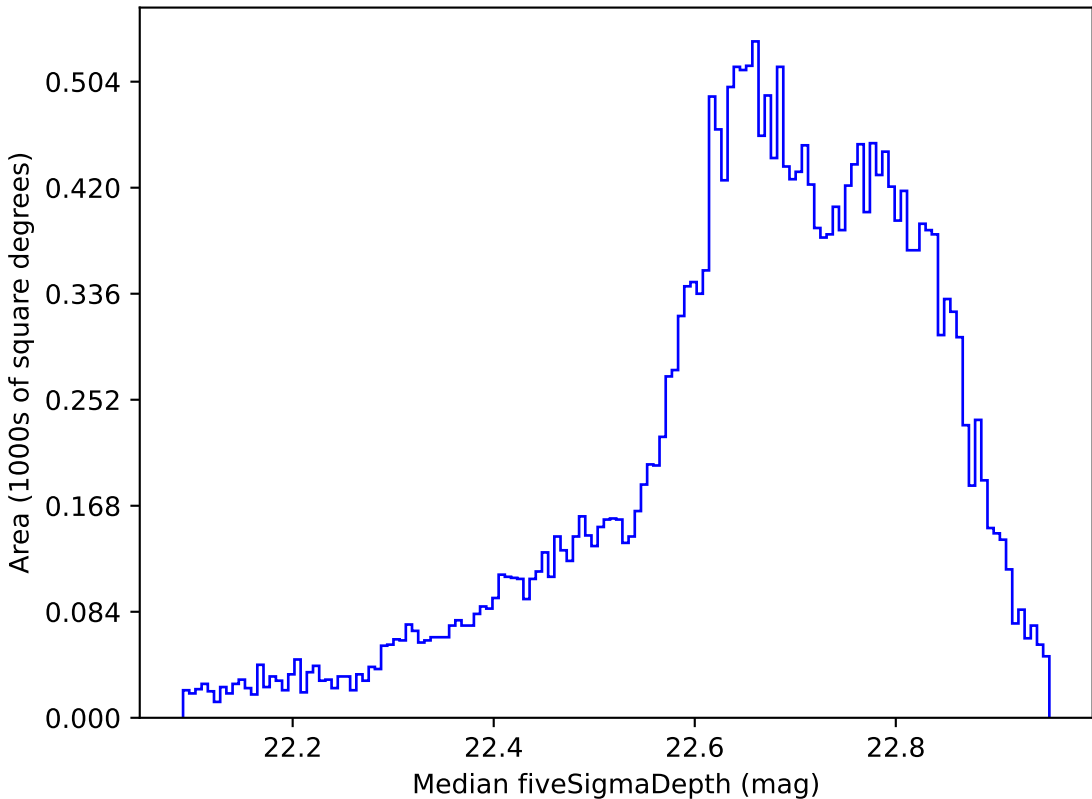
baseline_v2.1_10yrs All sky z band: Median fiveSigmaDepth
