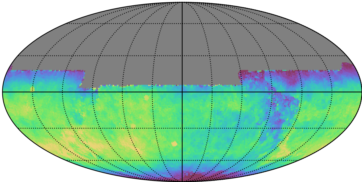
baseline_v2.1_10yrs All sky y band: Median fiveSigmaDepth
