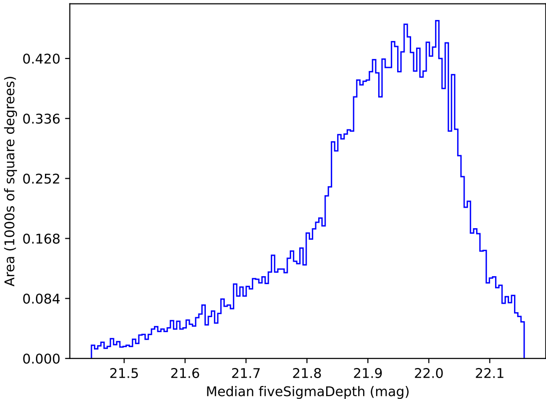
baseline_v2.1_10yrs All sky y band: Median fiveSigmaDepth
