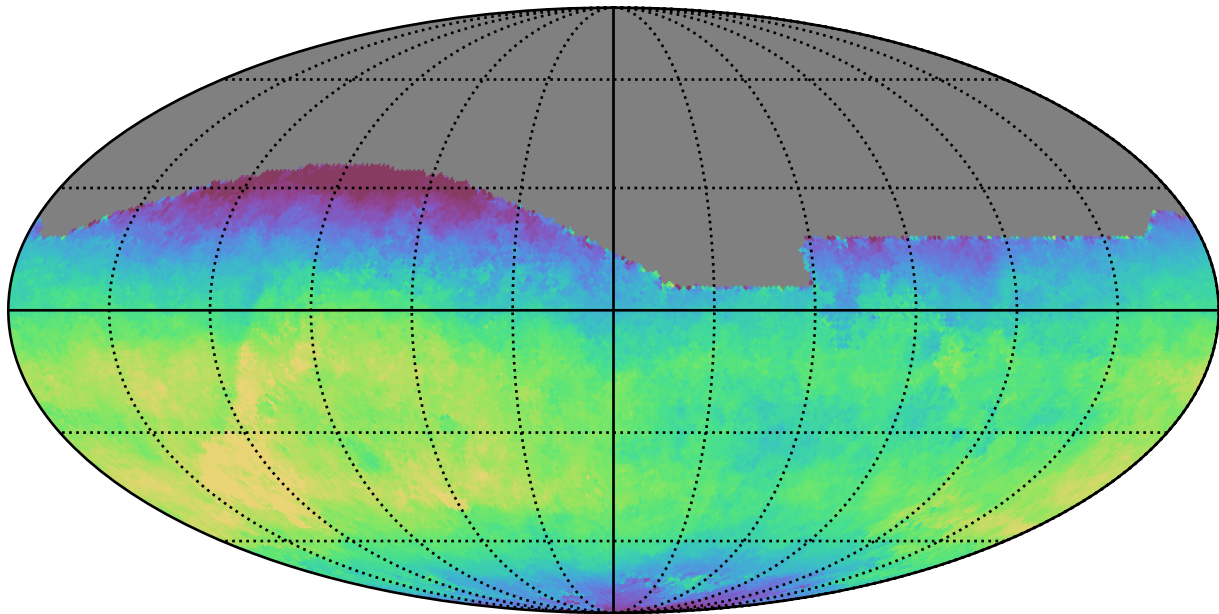
baseline_v2.1_10yrs All sky r band: Median fiveSigmaDepth
