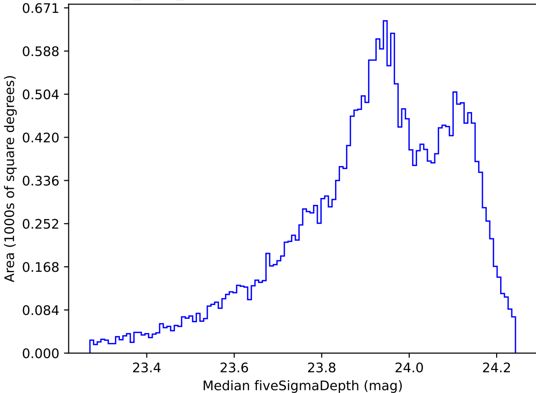
baseline_v2.1_10yrs All sky r band: Median fiveSigmaDepth
