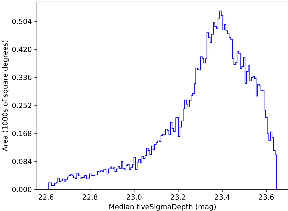
baseline_v2.1_10yrs All sky i band: Median fiveSigmaDepth
