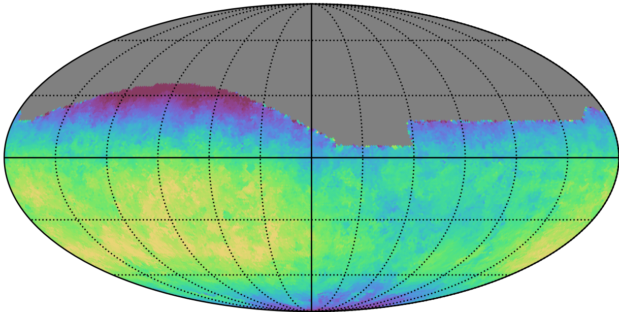
baseline_v2.1_10yrs All sky g band: Median fiveSigmaDepth
