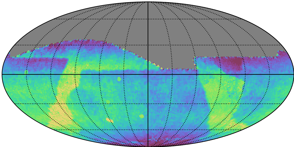
baseline_v2.1_10yrs All sky all bands: Median fiveSigmaDepth
