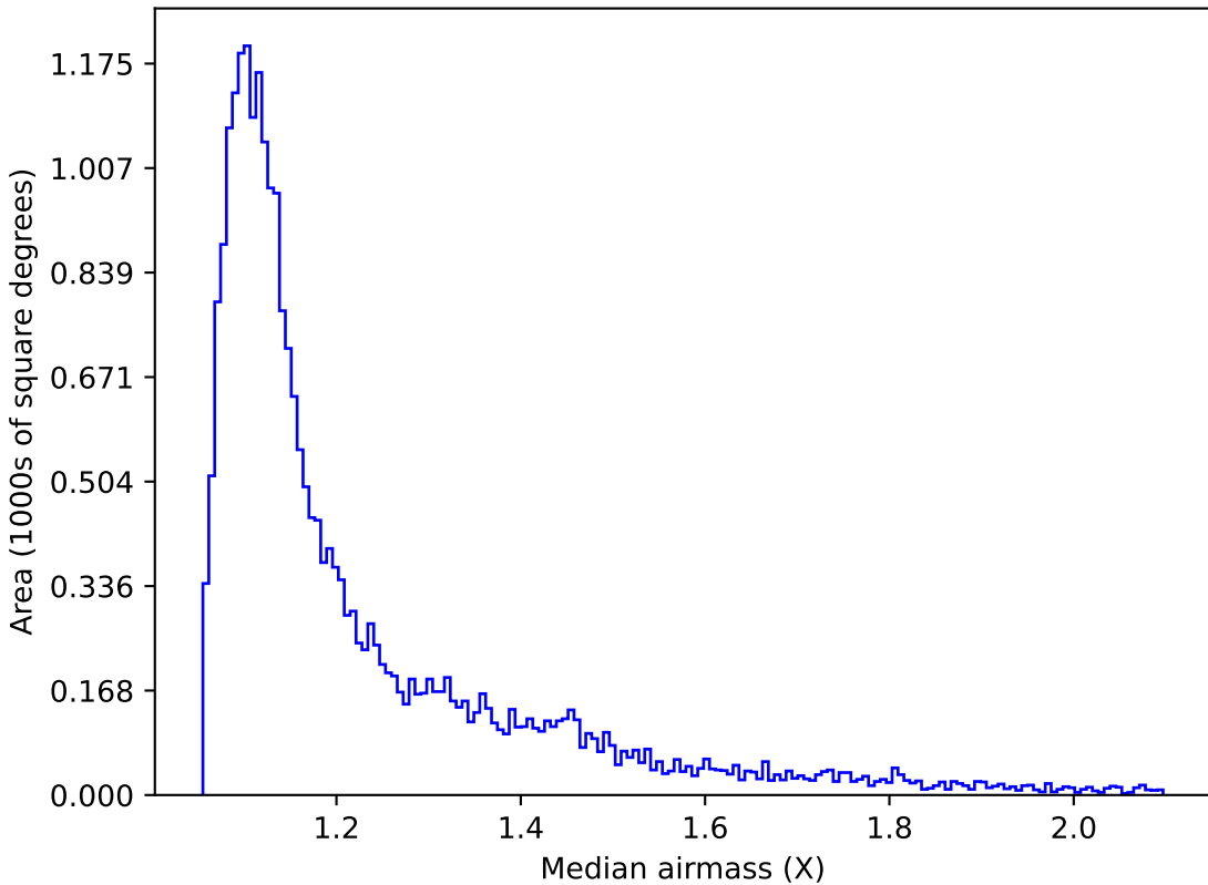
baseline_v2.1_10yrs Yr 1 z band: Median airmass
