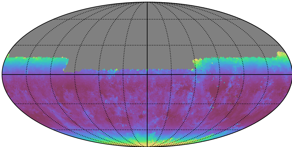
baseline_v2.1_10yrs Yr 1 y band: Median airmass
