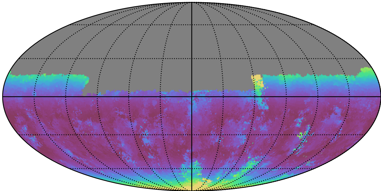
baseline_v2.1_10yrs Yr 1 u band: Median airmass
