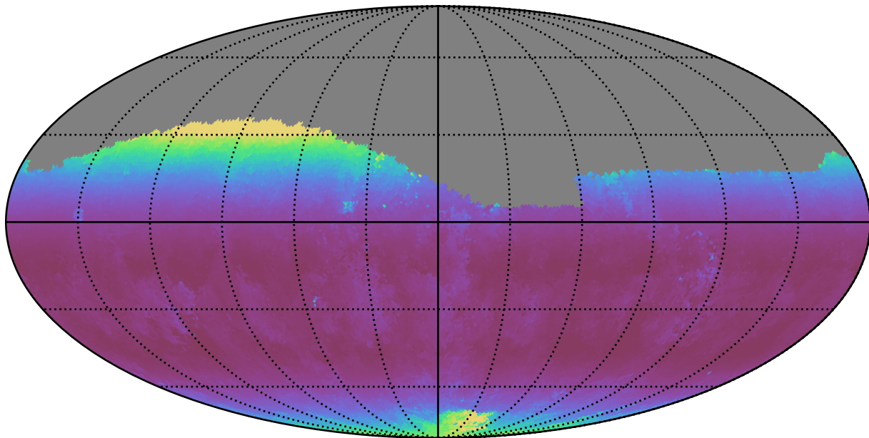
baseline_v2.1_10yrs Yr 1 r band: Median airmass
