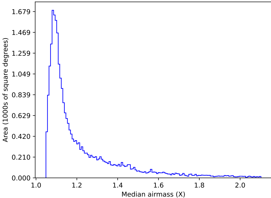
baseline_v2.1_10yrs Yr 1 r band: Median airmass
