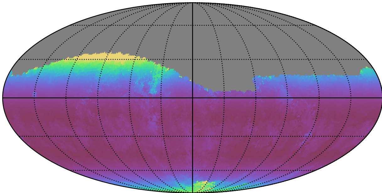
baseline_v2.1_10yrs Yr 1 i band: Median airmass
