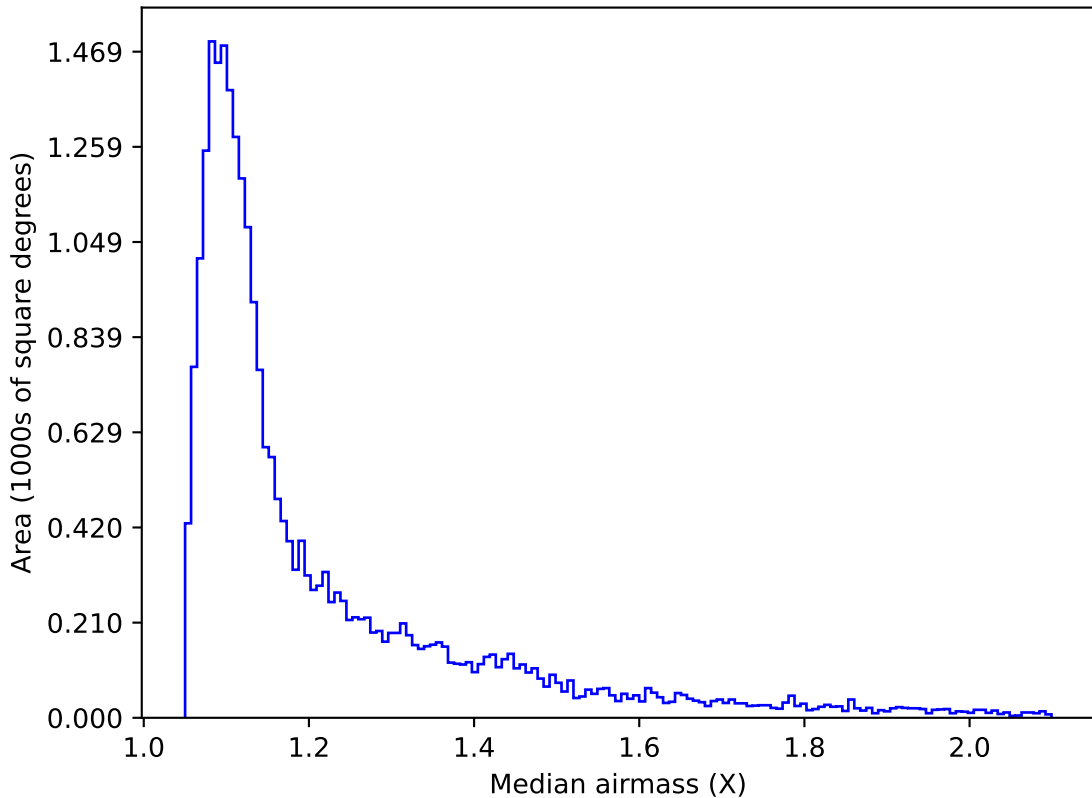
baseline_v2.1_10yrs Yr 1 i band: Median airmass
