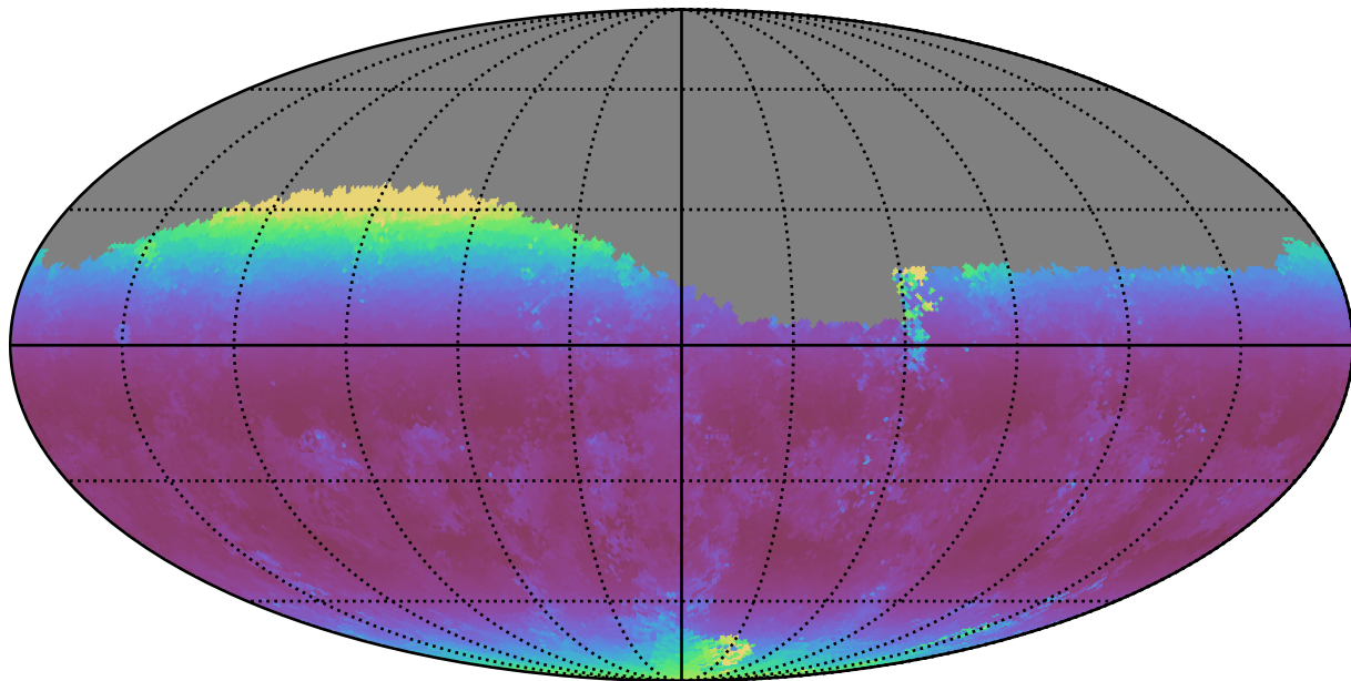
baseline_v2.1_10yrs Yr 1 g band: Median airmass
