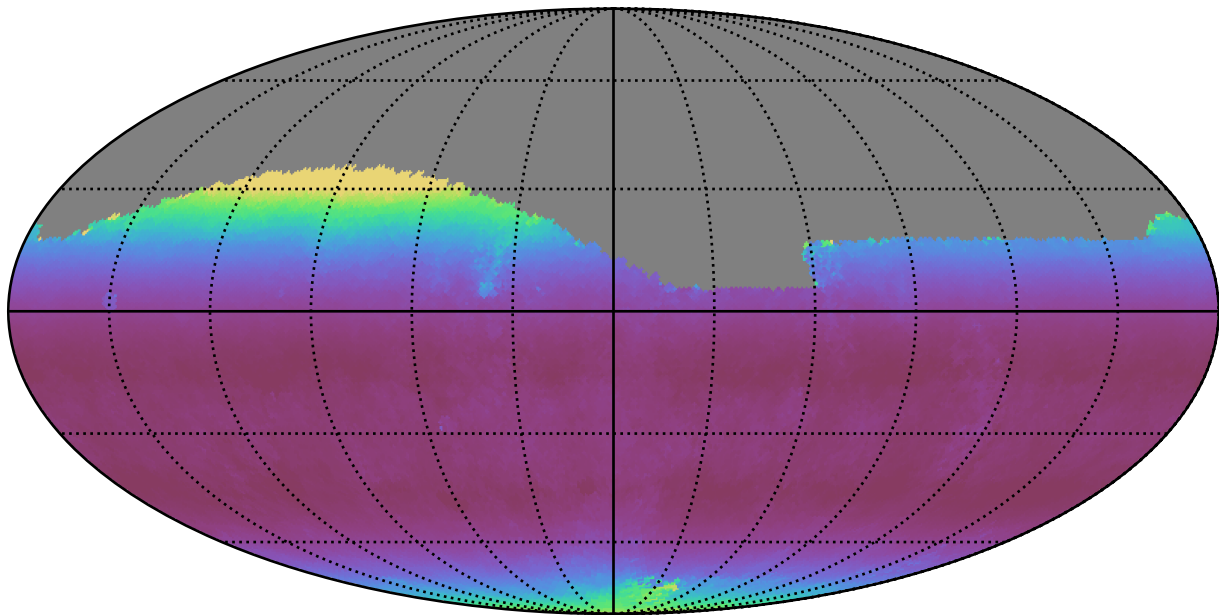
baseline_v2.1_10yrs Yr 1 all bands: Median airmass
