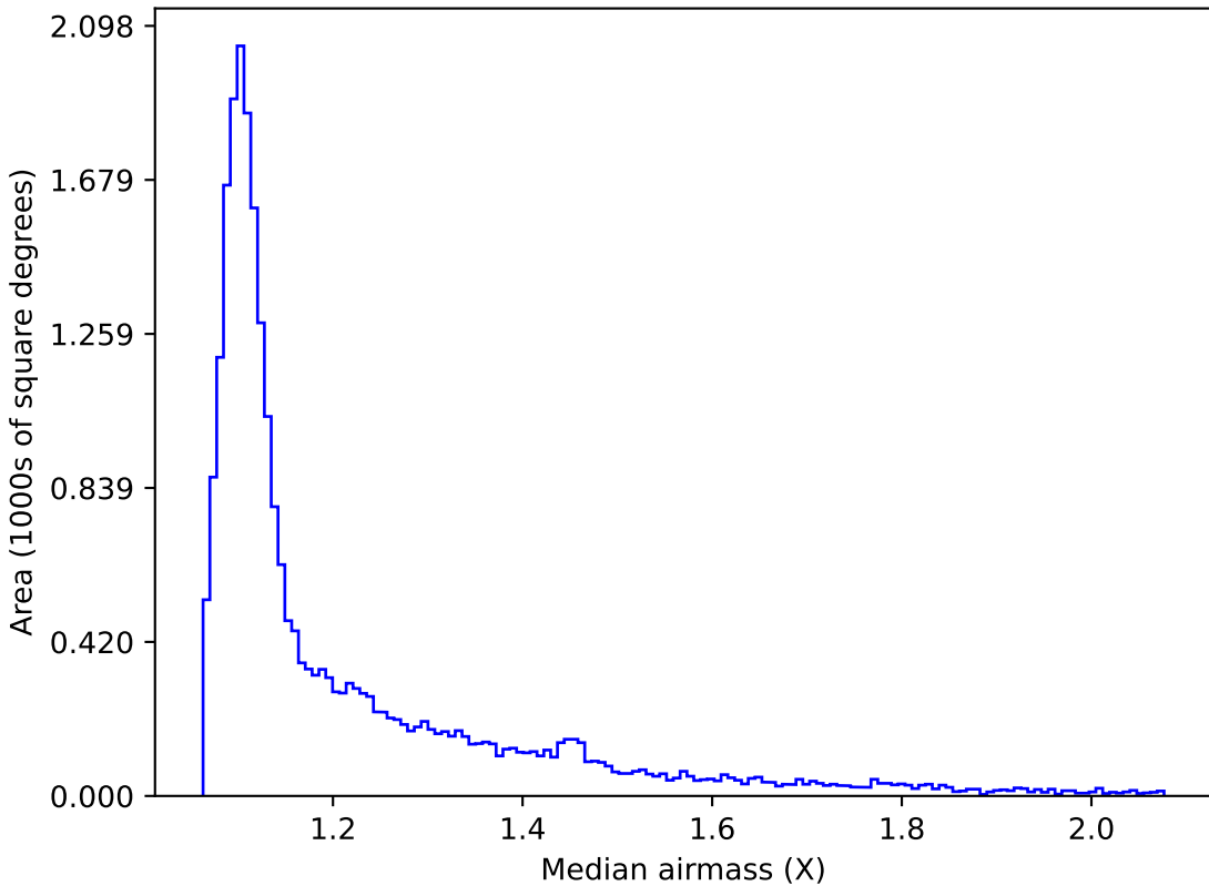
baseline_v2.1_10yrs Yr 1 all bands: Median airmass
