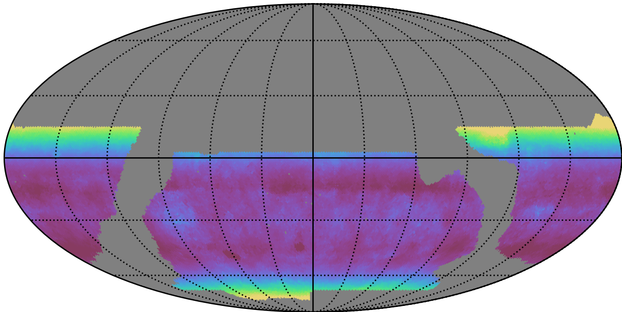
baseline_v2.1_10yrs WFD z band: Median airmass
