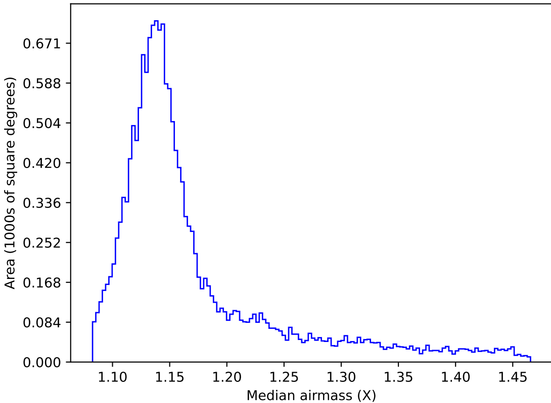
baseline_v2.1_10yrs WFD z band: Median airmass
