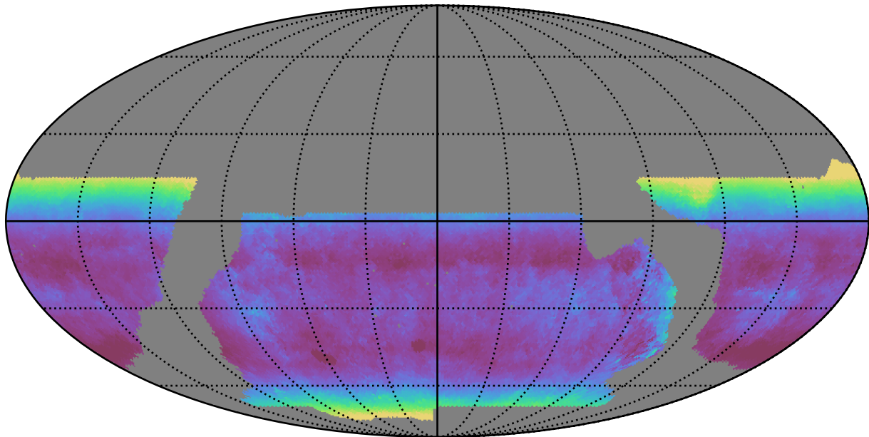
baseline_v2.1_10yrs WFD y band: Median airmass
