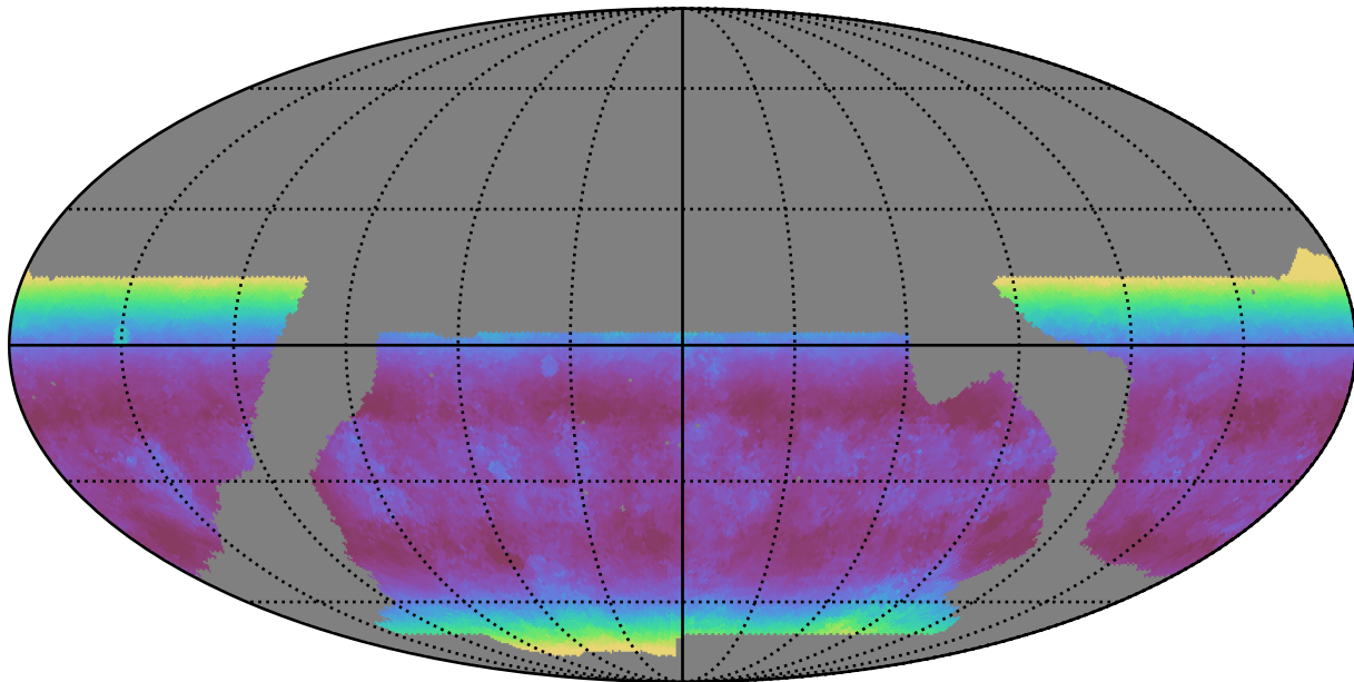
baseline_v2.1_10yrs WFD u band: Median airmass
