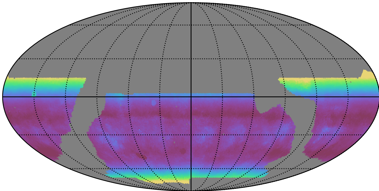
baseline_v2.1_10yrs WFD r band: Median airmass
