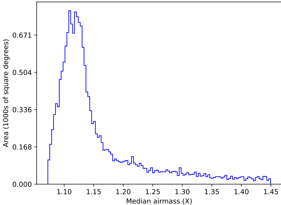
baseline_v2.1_10yrs WFD r band: Median airmass
