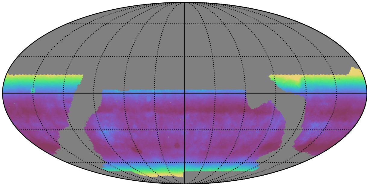
baseline_v2.1_10yrs WFD i band: Median airmass
