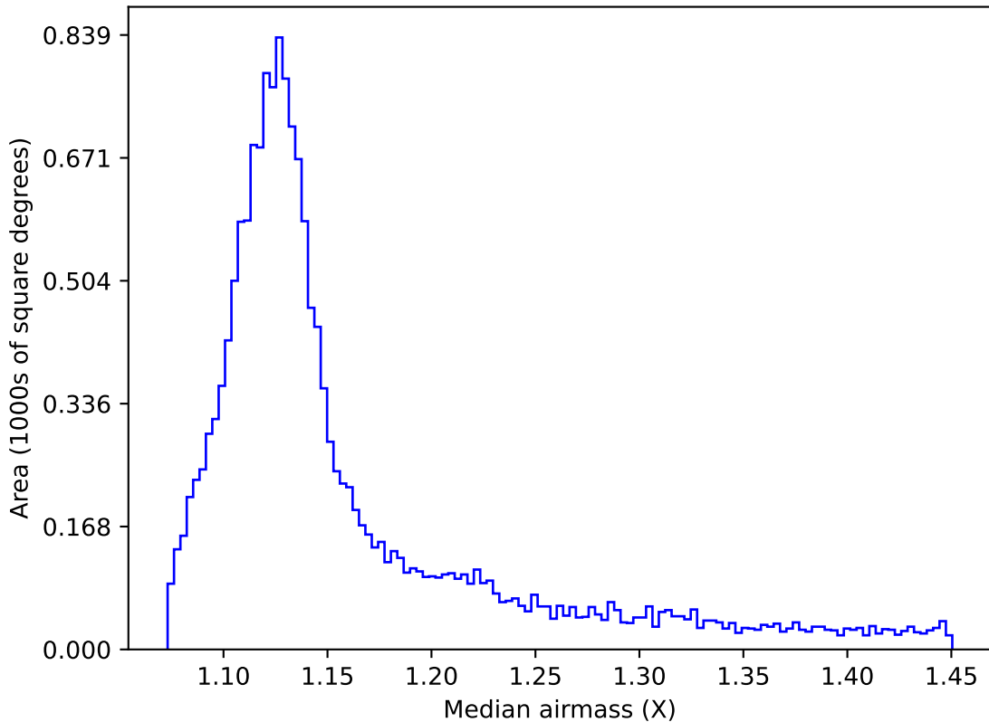
baseline_v2.1_10yrs WFD i band: Median airmass
