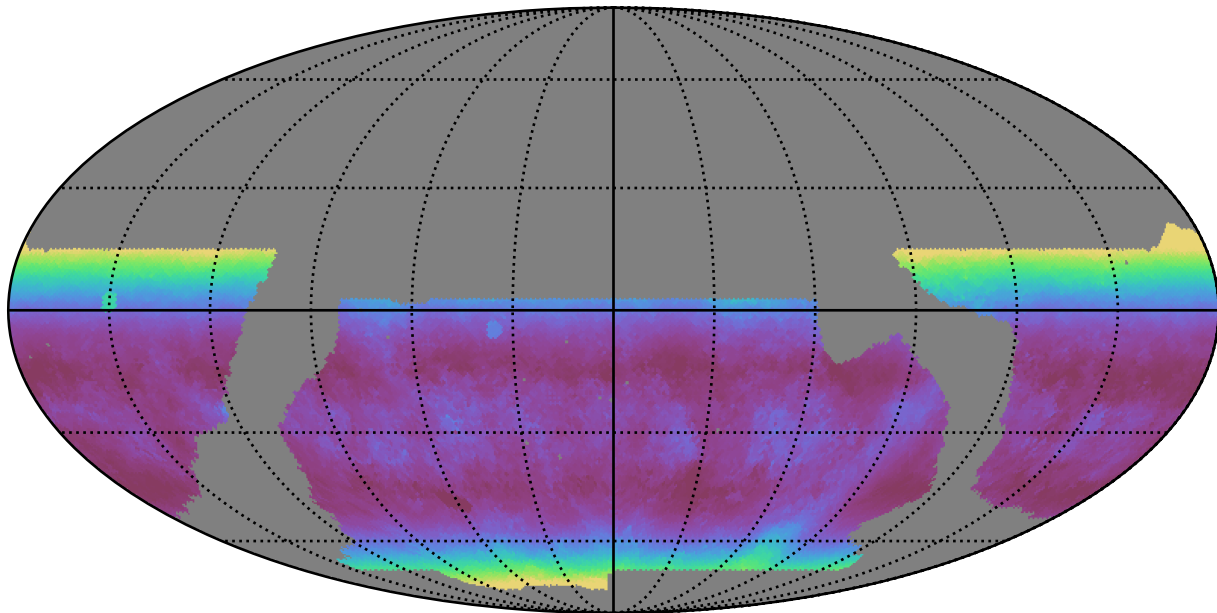
baseline_v2.1_10yrs WFD g band: Median airmass
