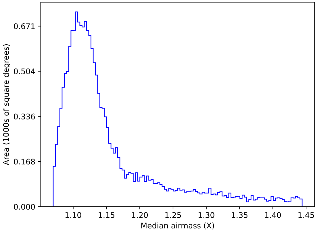
baseline_v2.1_10yrs WFD g band: Median airmass
