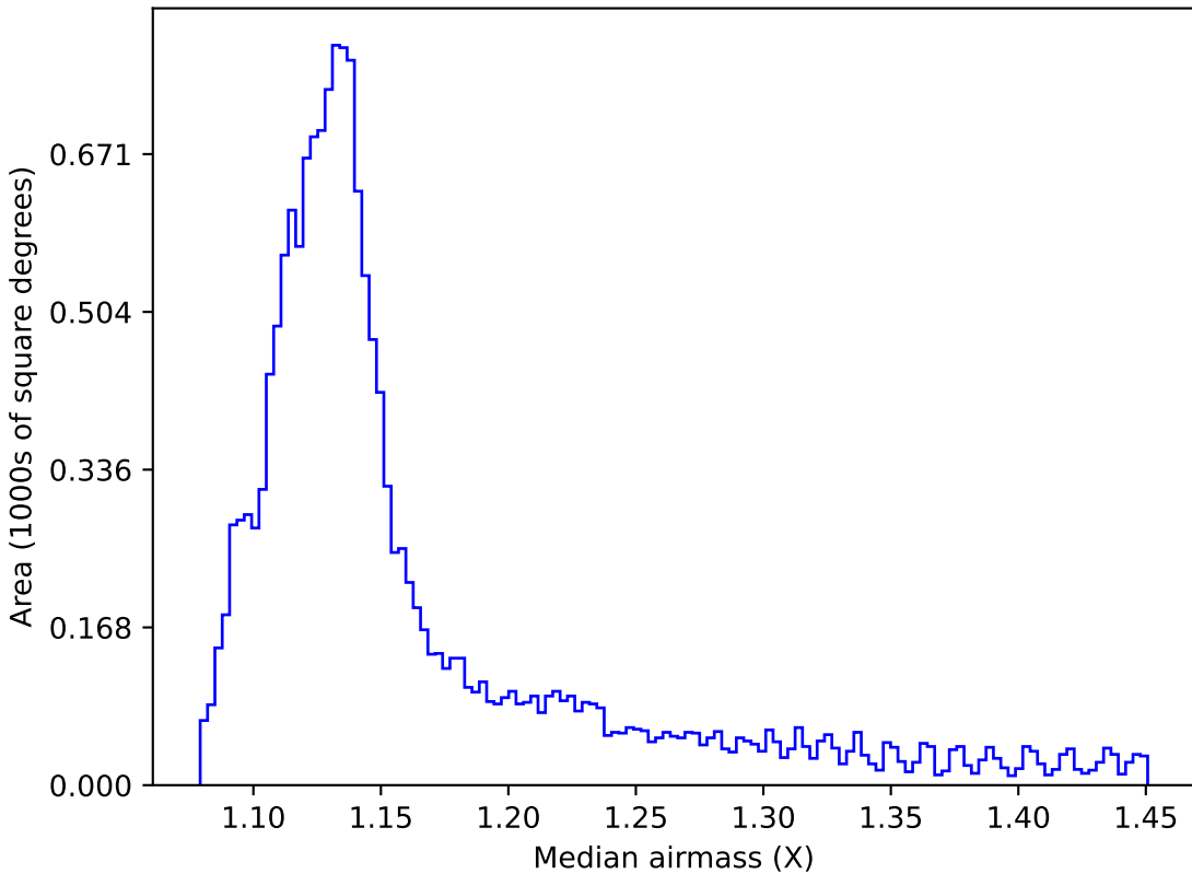
baseline_v2.1_10yrs WFD all bands: Median airmass
