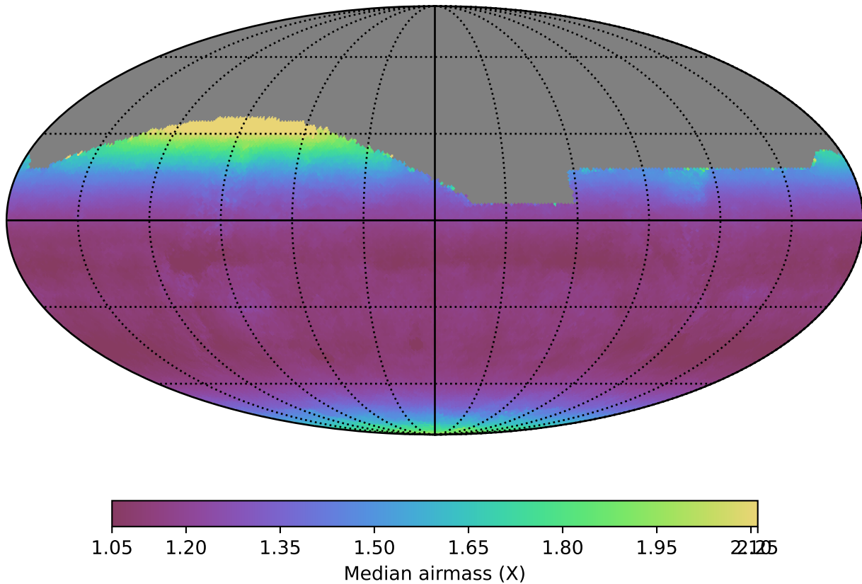
baseline_v2.1_10yrs All sky z band: Median airmass
