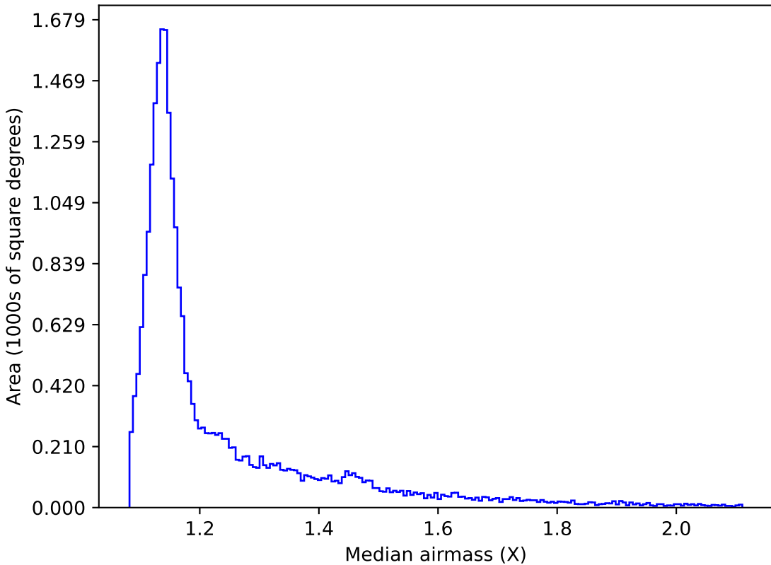
baseline_v2.1_10yrs All sky z band: Median airmass
