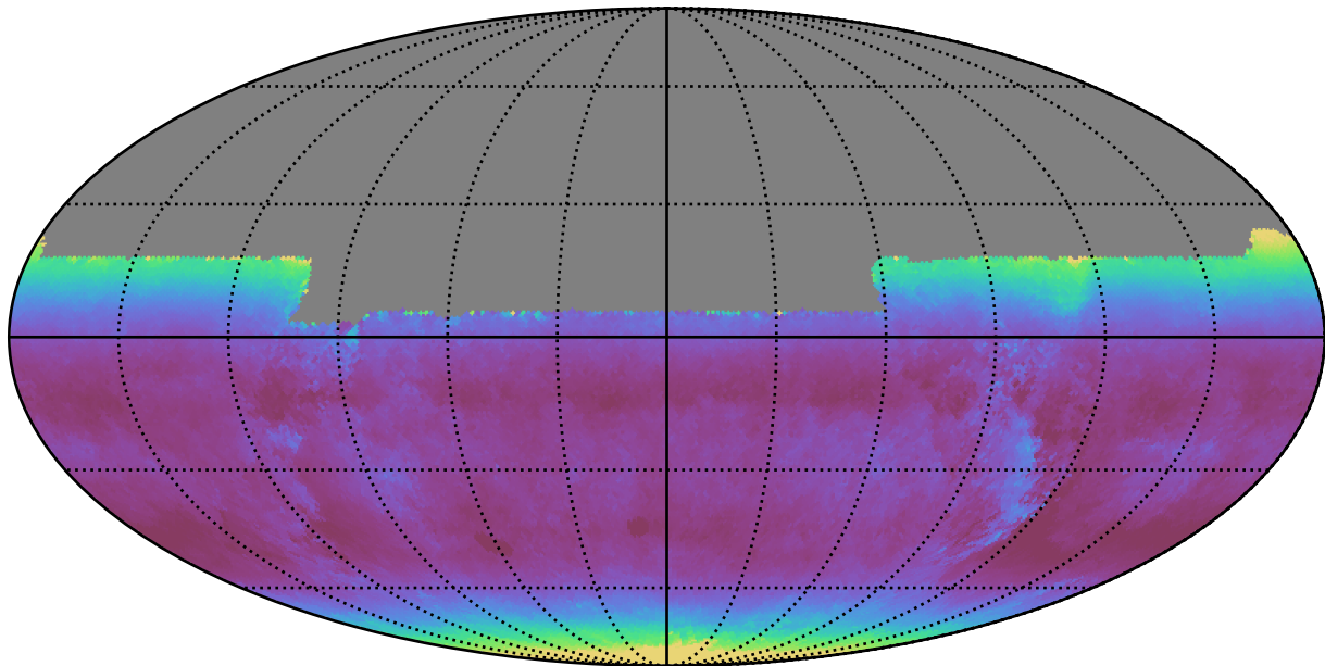
baseline_v2.1_10yrs All sky y band: Median airmass
