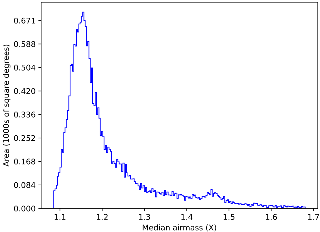
baseline_v2.1_10yrs All sky y band: Median airmass
