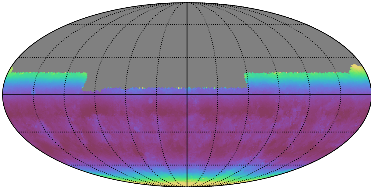
baseline_v2.1_10yrs All sky u band: Median airmass
