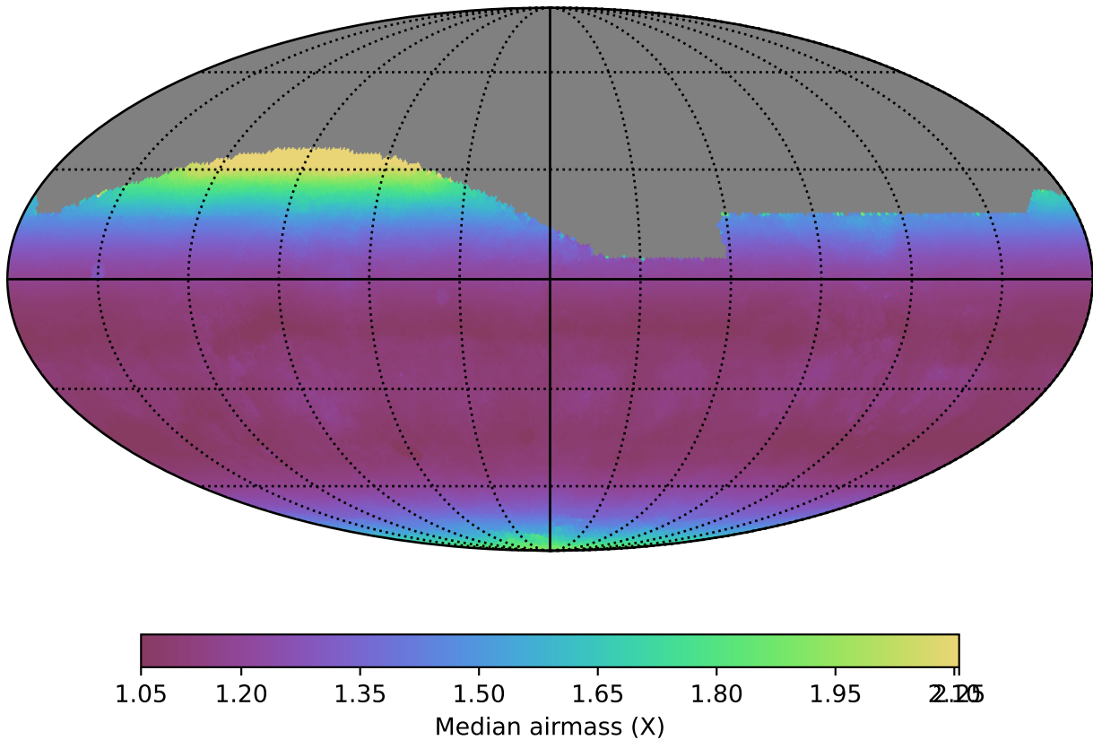
baseline_v2.1_10yrs All sky r band: Median airmass
