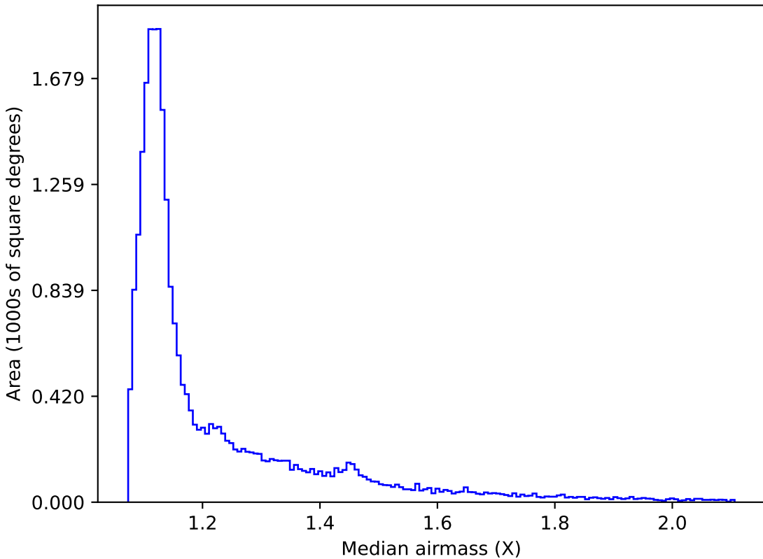
baseline_v2.1_10yrs All sky r band: Median airmass
