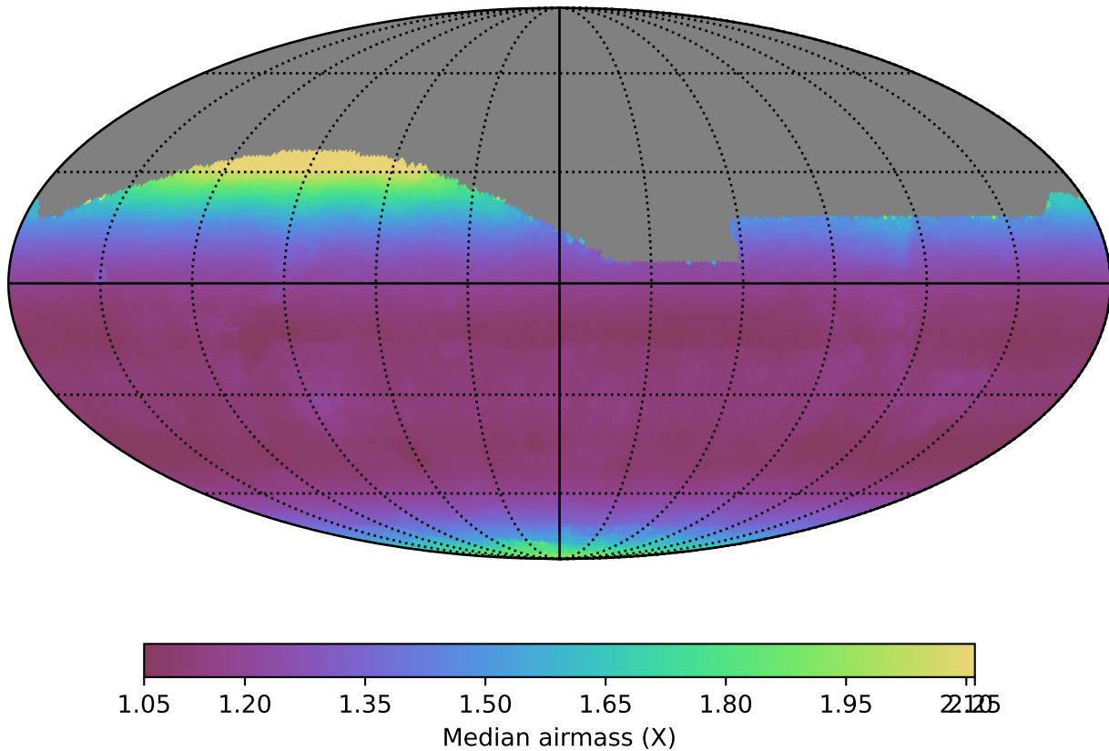
baseline_v2.1_10yrs All sky i band: Median airmass
