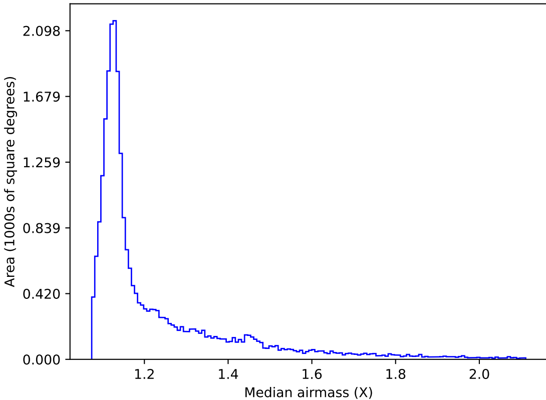
baseline_v2.1_10yrs All sky i band: Median airmass
