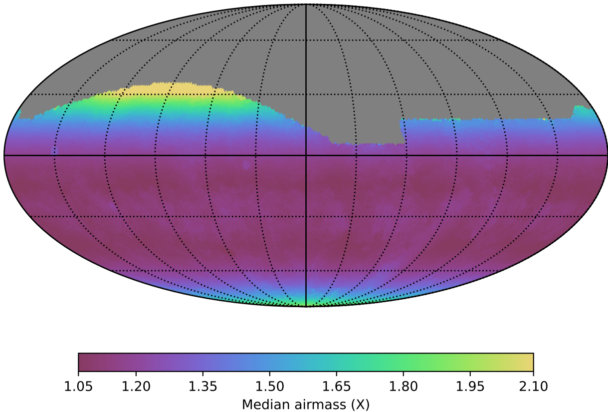
baseline_v2.1_10yrs All sky g band: Median airmass
