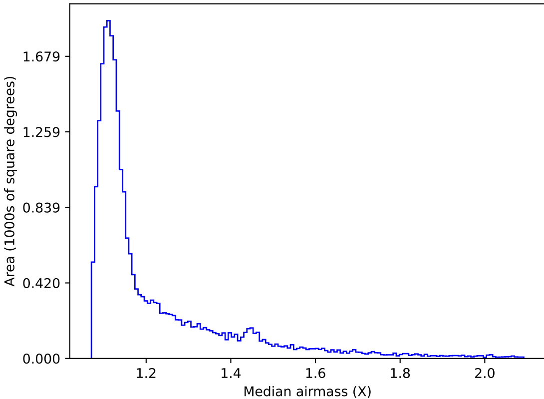
baseline_v2.1_10yrs All sky g band: Median airmass
